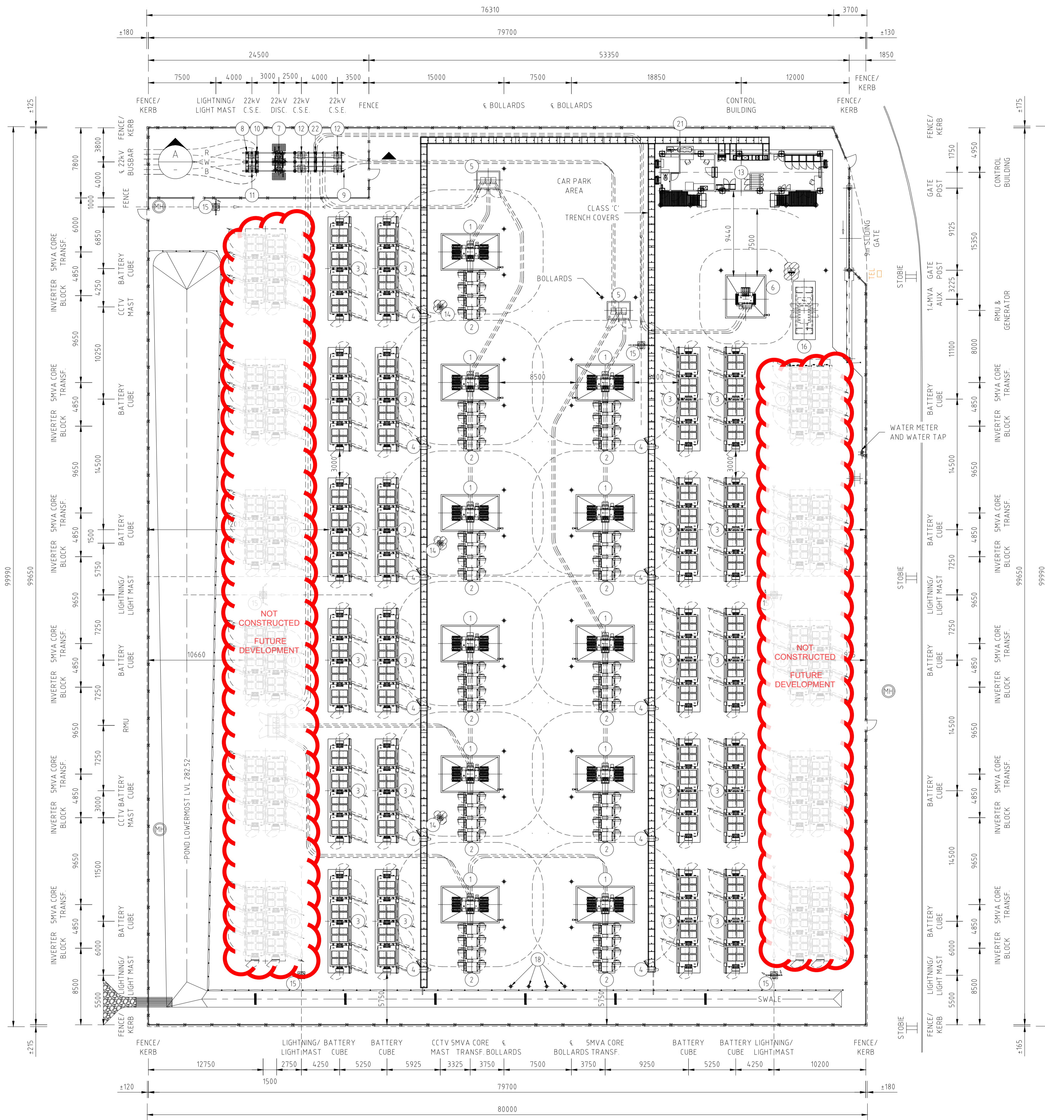
PLAN VIEW BROKEN HILL BESS SCALE 1:250
