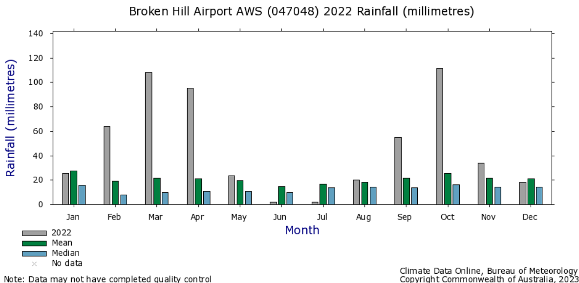
Figure 2.3: Rainfall in Broken Hill in 2022 (source: Australian Bureau of Meteorology, 2023)
