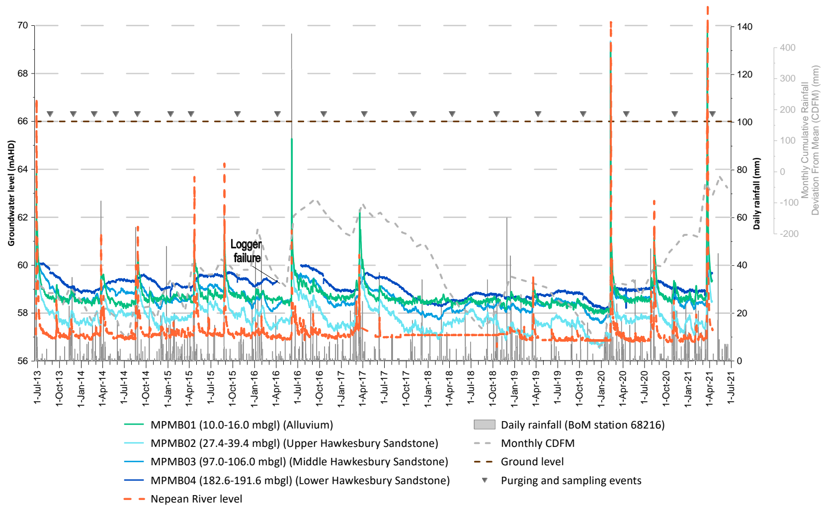
Figure 4.1 Groundwater levels at the Menangle Park site
