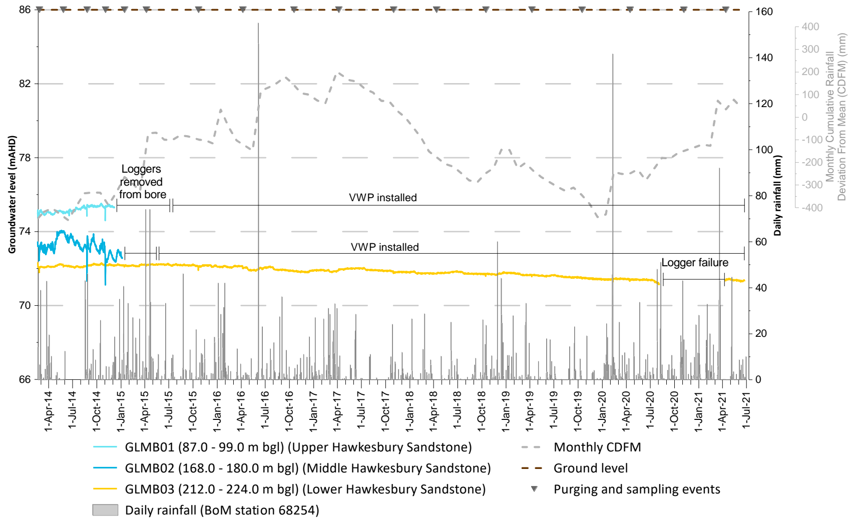
Figure 4.2 Groundwater levels at the Glenlee site
