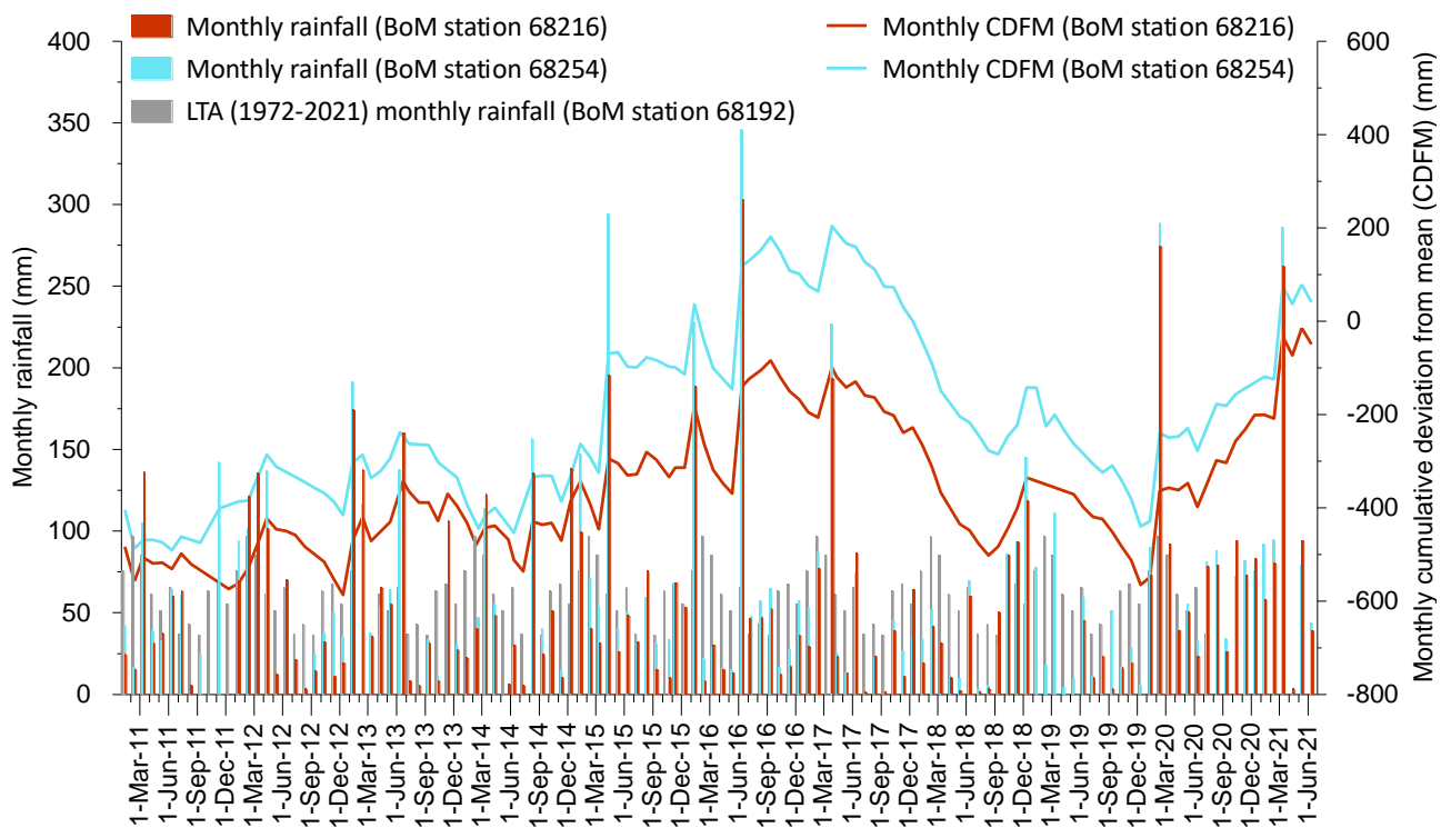
Figure 2.2 Monthly rainfall for the monitoring period (2011-2021)
