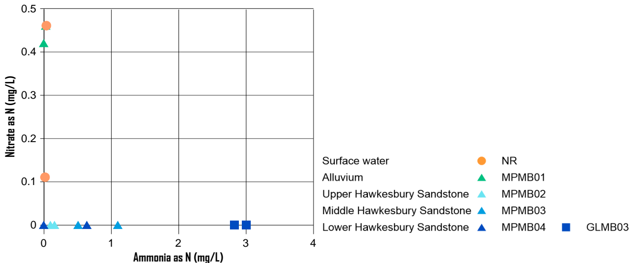
Figure 5.5 Ammonia versus nitrate concentrations in groundwater for CGP monitoring bores (2020/21 monitoring year)
