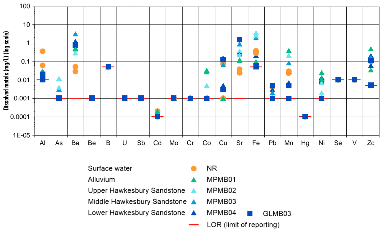
Figure 5.4 Dissolved metal concentrations in groundwater for CGP monitoring bores (2020/21 monitoring year)
