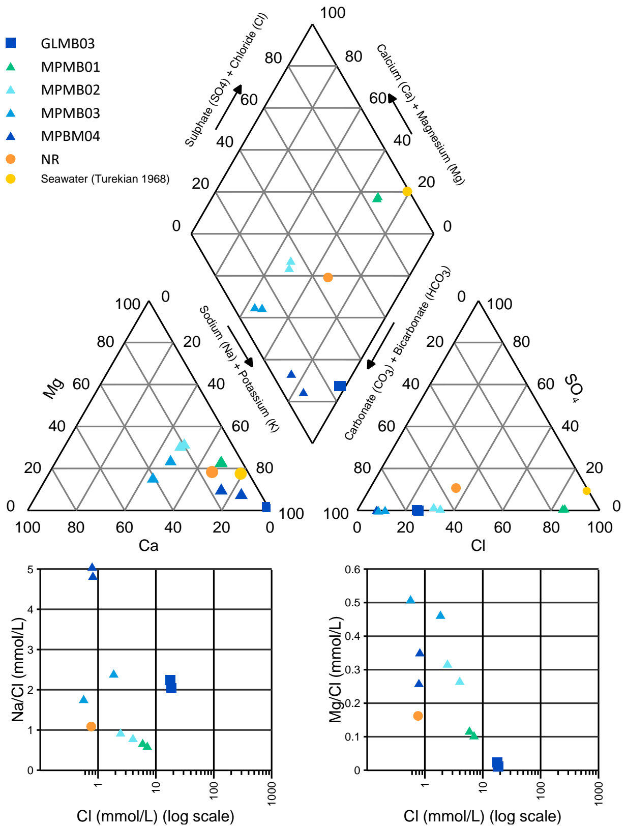
Figure 5.3 Major ion chemistry of groundwater for CGP monitoring bores (2020/21 monitoring year)
