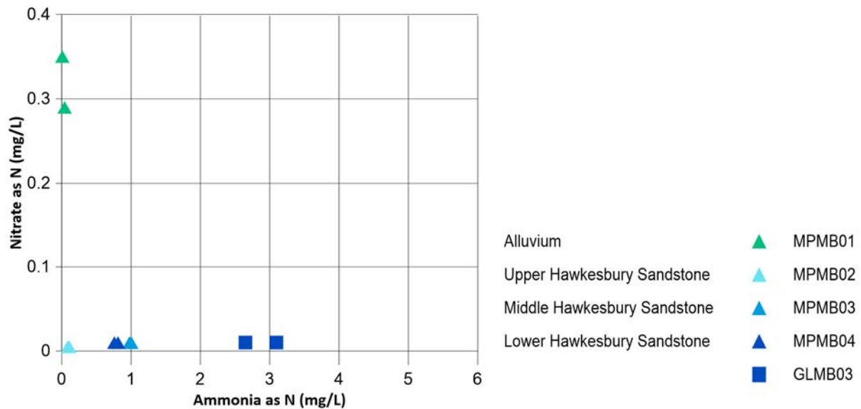
Figure 5.5 Ammonia versus nitrate concentrations in groundwater for CGP monitoring bores (2017/18 monitoring year)
