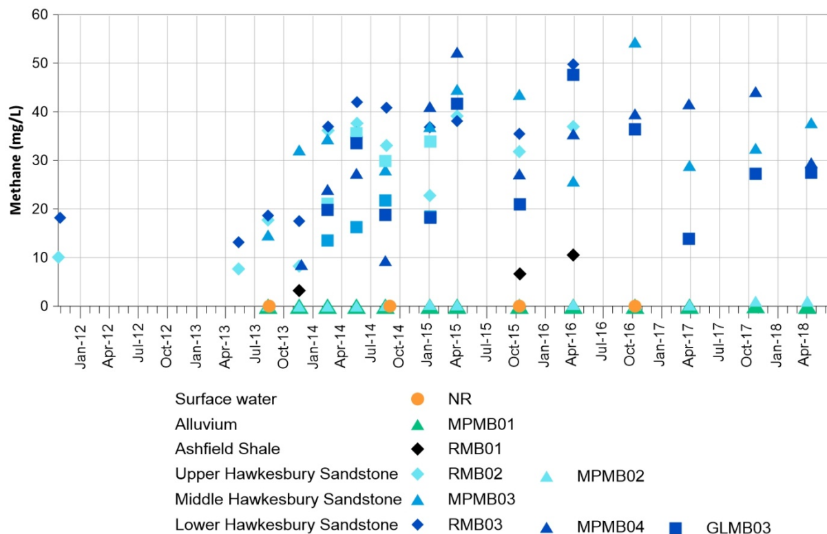
Figure 5.6 Dissolved methane time series for CGP monitoring bores and Nepean River samples
