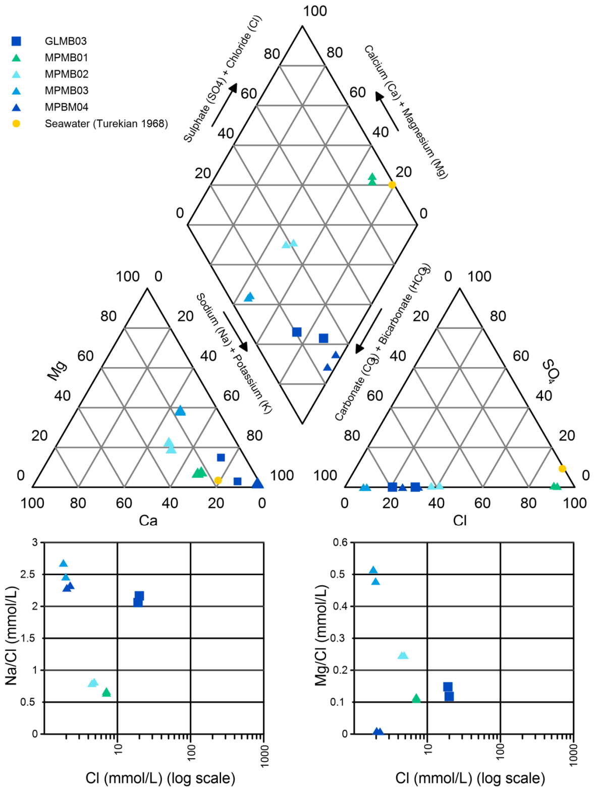
Figure 5.3 Major ion chemistry of groundwater for CGP monitoring bores (2017/18 monitoring year)
