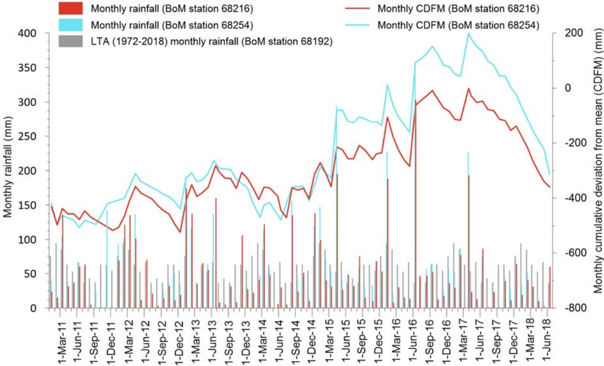
Figure 2.2 Monthly rainfall for the monitoring period (2011 – 2018)
