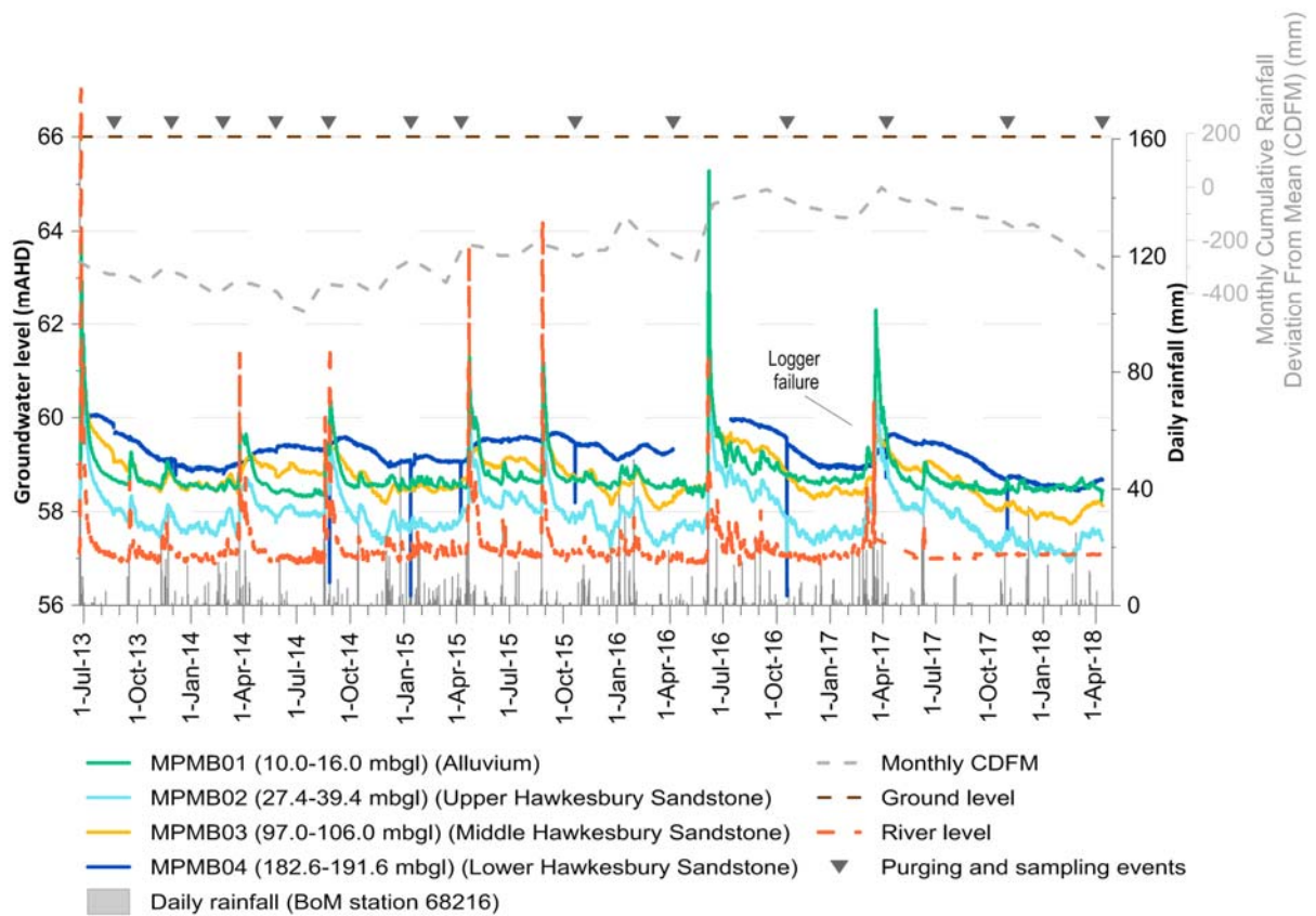
Figure 4.1 Groundwater levels at the Menangle Park site
