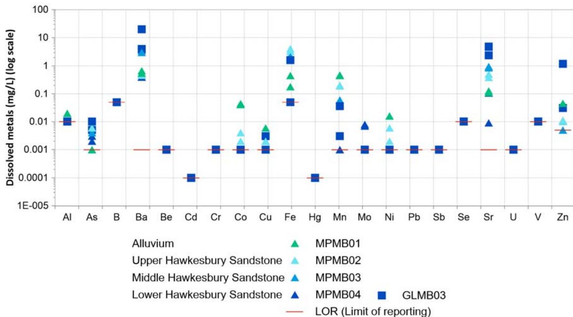
Figure 5.4 Dissolved metal concentrations in groundwater for CGP monitoring bores (2017/18 monitoring year)
