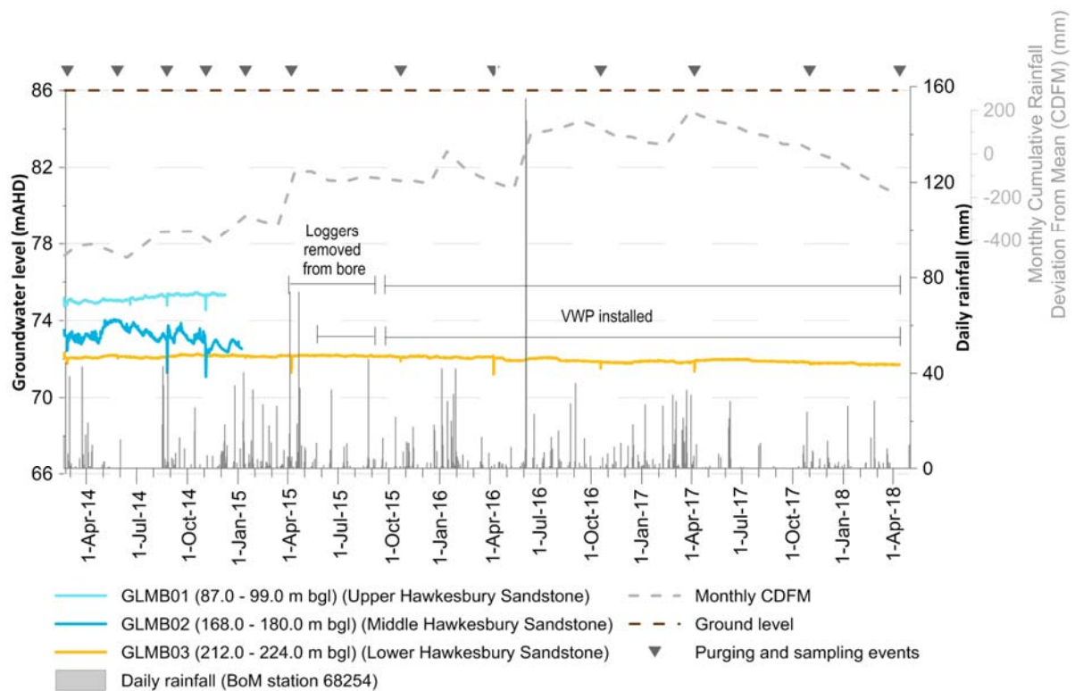
Figure 4.2 Groundwater levels at the Glenlee site
