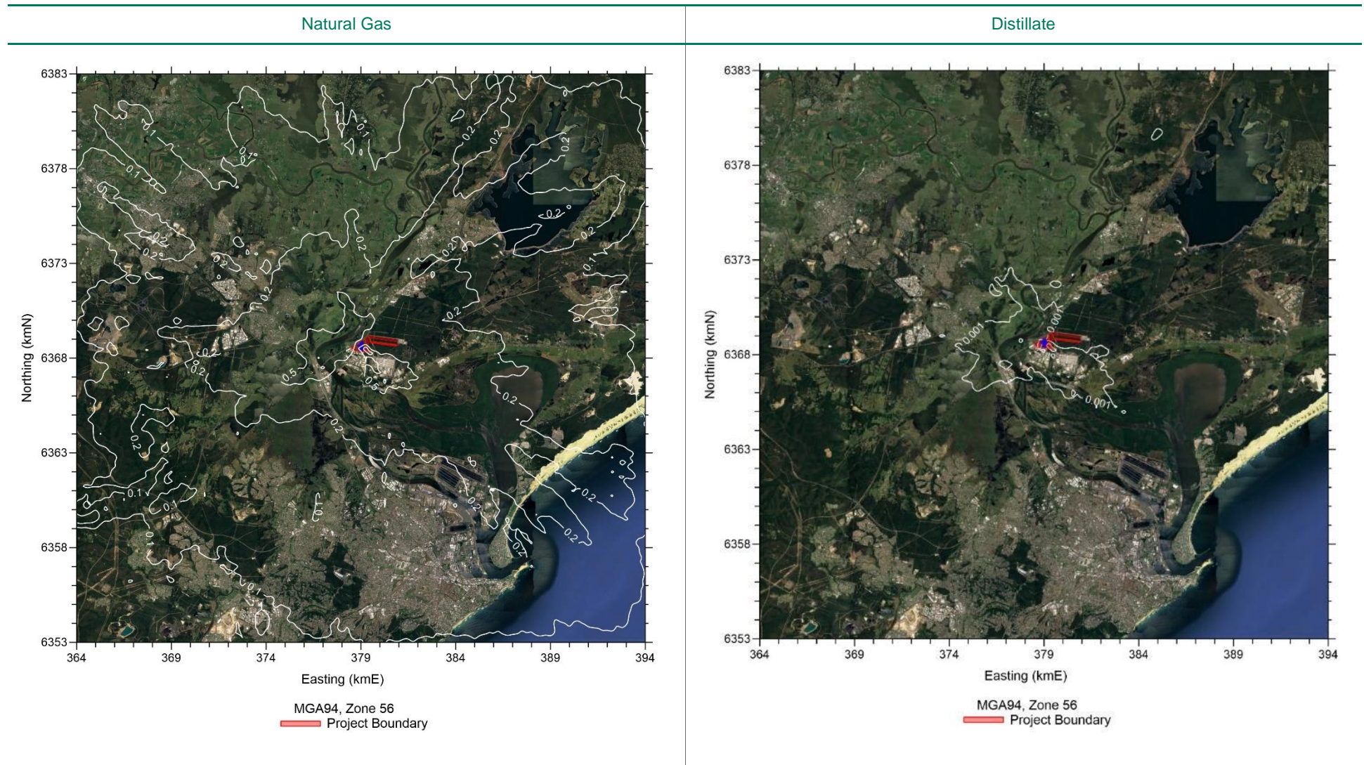
Figure 7.10: 99.9 th percentile incremental 1 hour average acrolein predictions – Reciprocating Engine Option ( \mu\text{g}/\text{m}^3 )
