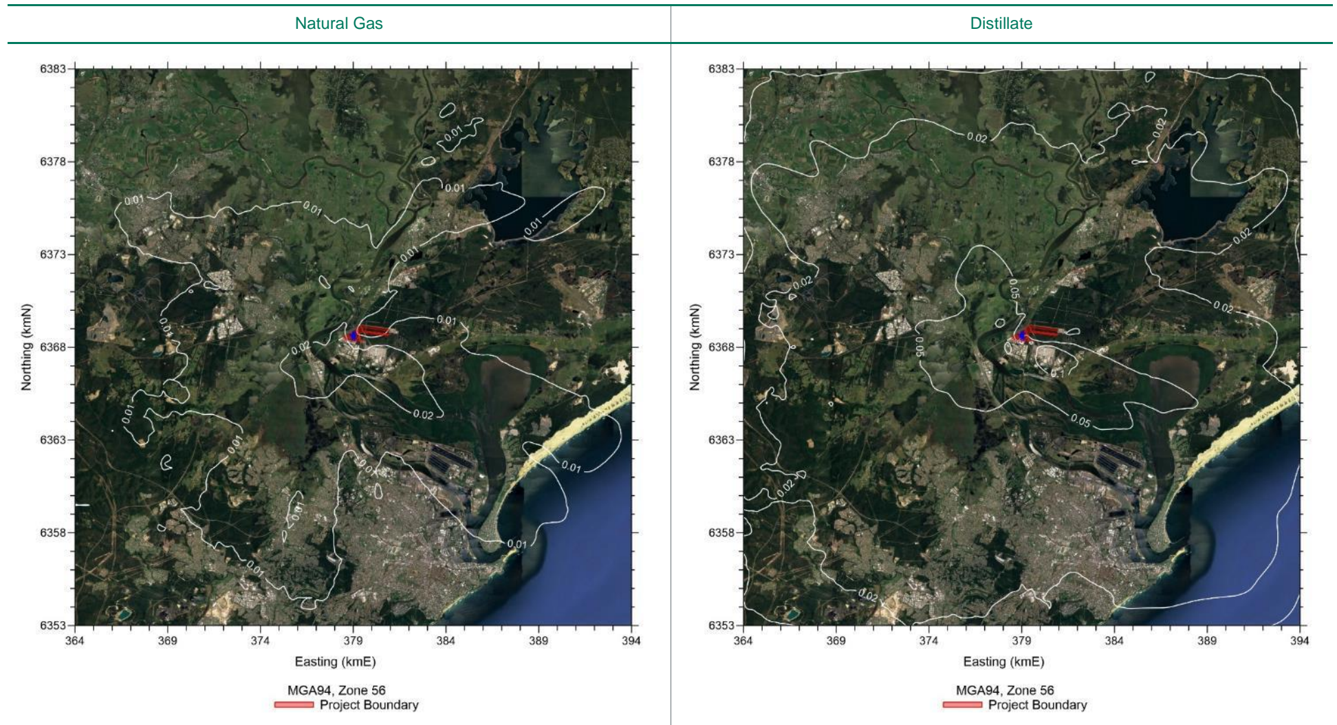
Figure 7.7: Incremental annual average PM 2.5 predictions – Gas Turbine Option (µg/m 3 )
