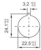
SHML Version
